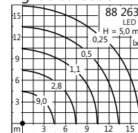
Light distribution
